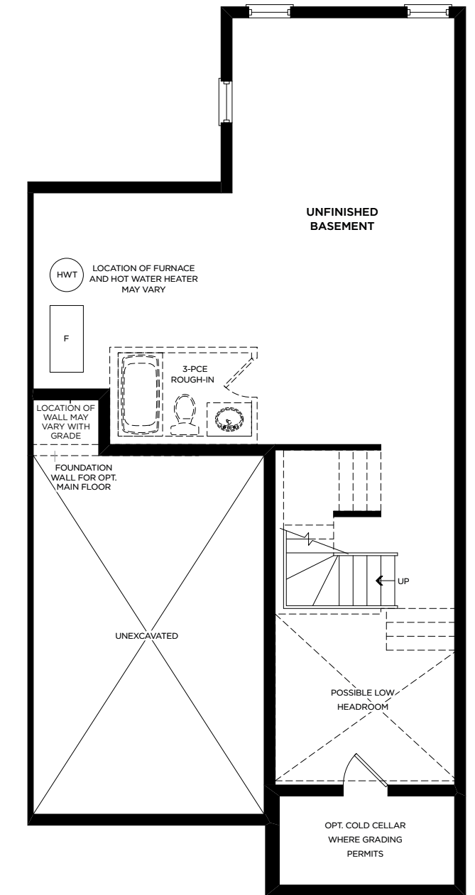
BASEMENT ELEVATION A & B
