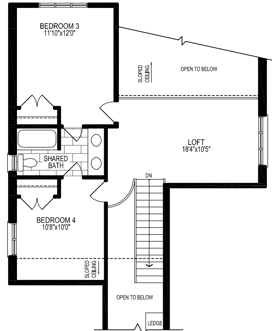
OPT. LOFT LEVEL STYLE A (B & C SIMILAR)
