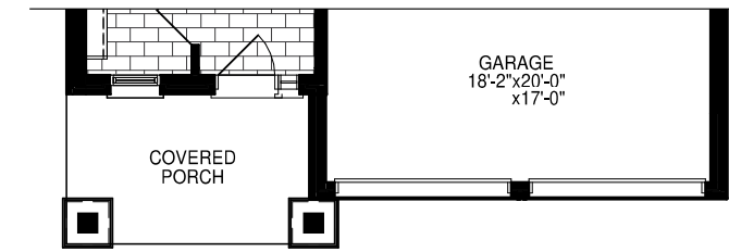
PART. MAIN LEVEL STYLE B
