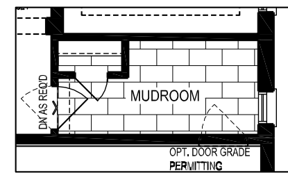
PART. MAIN LEVEL FOR OPT. SECOND LEVEL LAUNDRY STYLE A (B & C SIMILAR)
