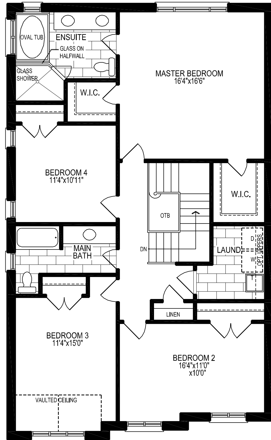
SECOND LEVEL STYLE A
