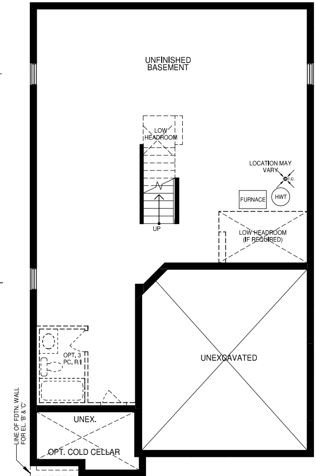
LOWER LEVEL STYLE A (B & C SIMILAR)
