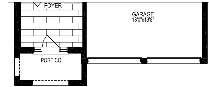
PART. MAIN LEVEL STYLE B
