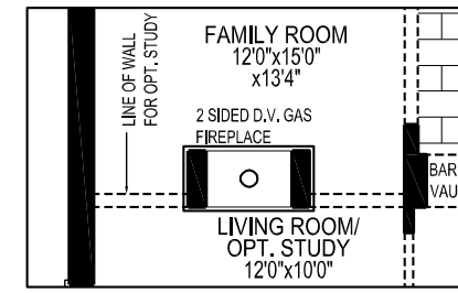
PART. OPT. MAIN LEVEL W/2-SIDED FIREPLACE STYLE A (B & C SIMILAR)
