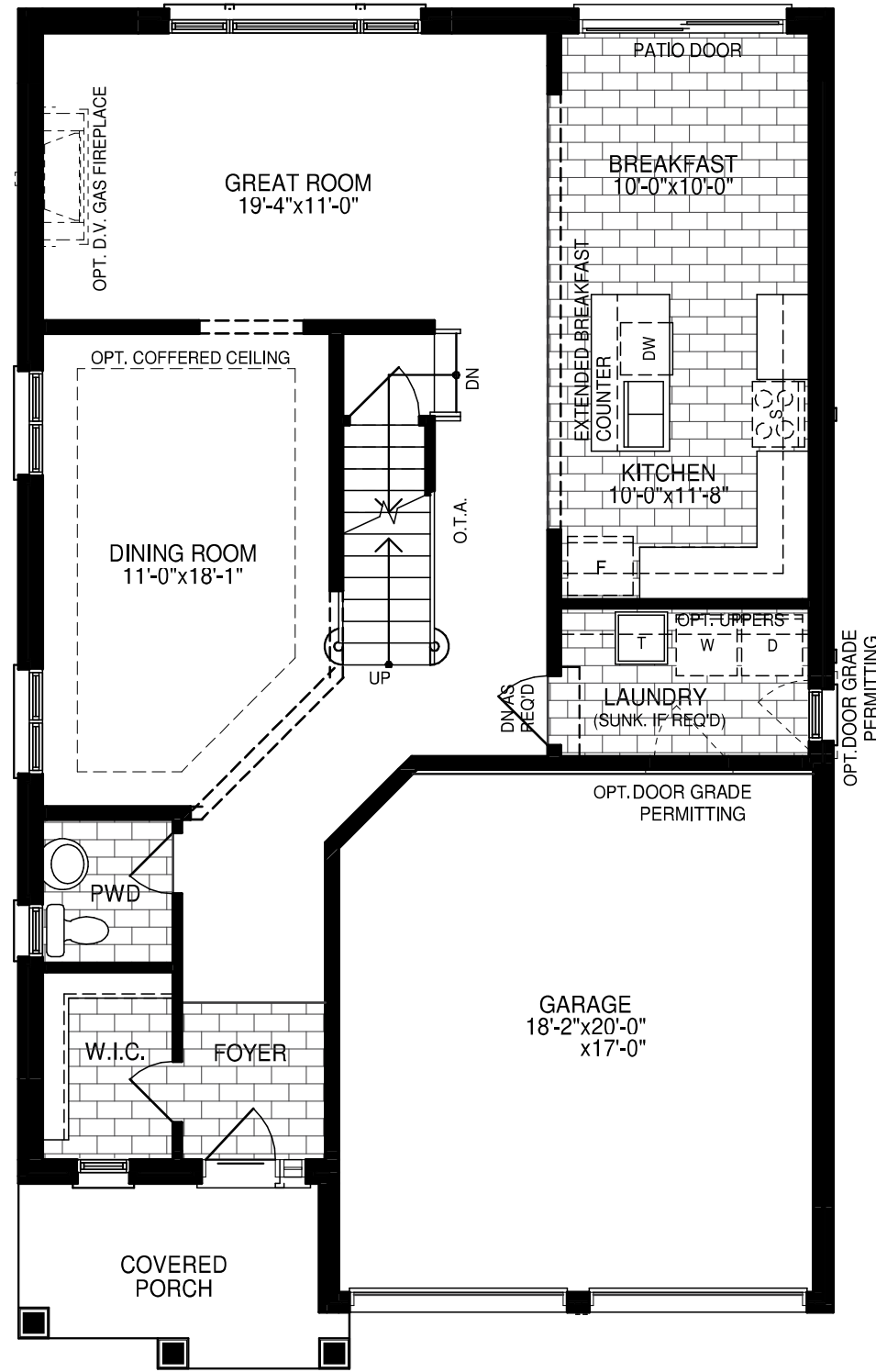
MAIN LEVEL STYLE A
