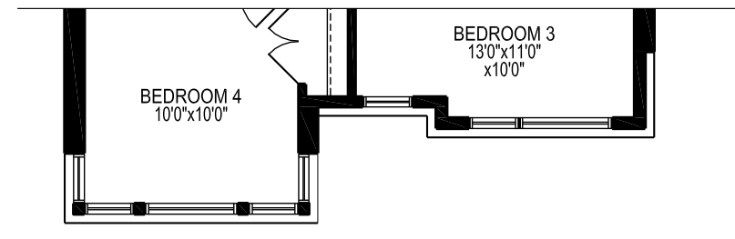
PART. SECOND LEVEL STYLE B
