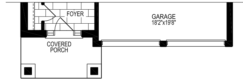
PART. MAIN LEVEL STYLE C
