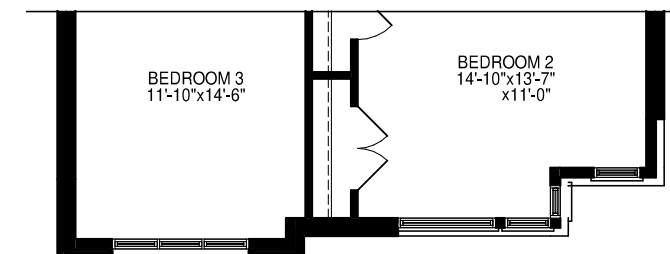
PART. SECOND LEVEL STYLE B
