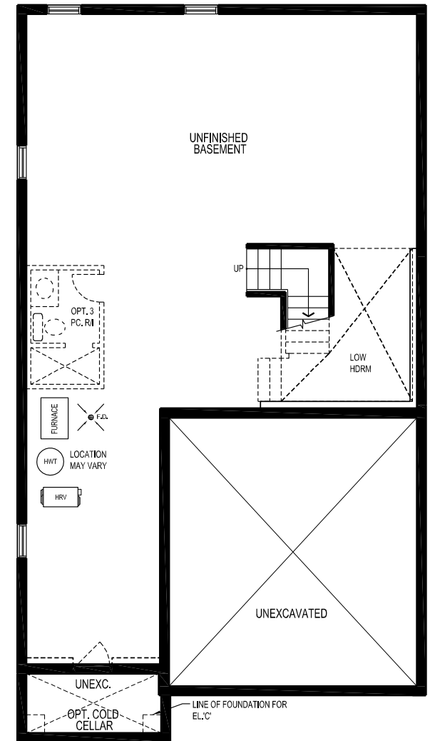
LOWER LEVEL STYLE A, B & C
