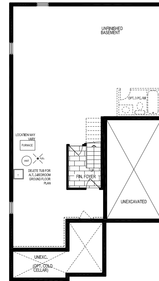
LOWER LEVEL STYLE A
