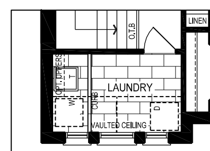
PART. OPT. SECOND LEVEL W/SECOND LEVEL LAUNDRY STYLE A (B & C SIMILAR)
