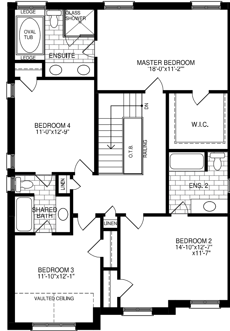
OPT. SECOND LEVEL STYLE A (B & C SIMILAR)
