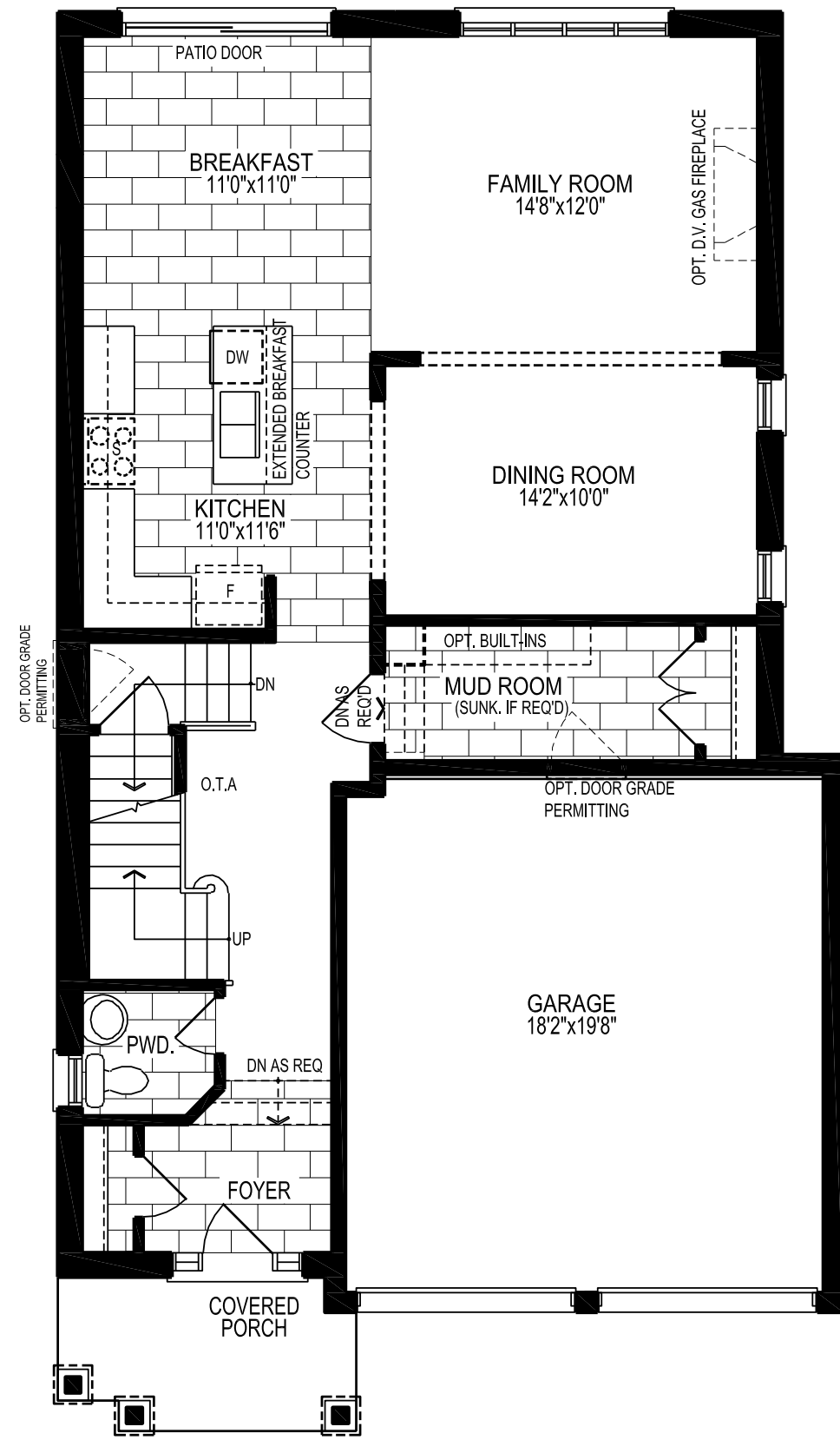
MAIN LEVEL STYLE A
