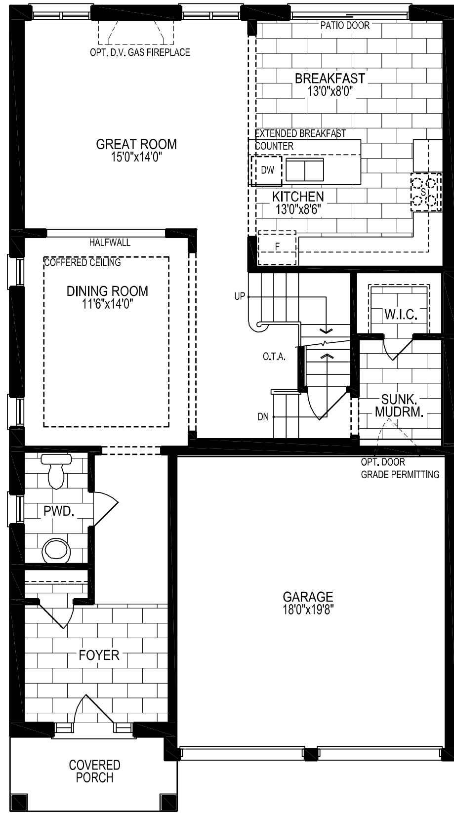
MAIN LEVEL STYLE A
