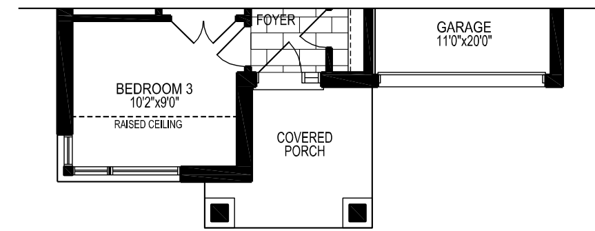
PART. MAIN LEVEL STYLE B
